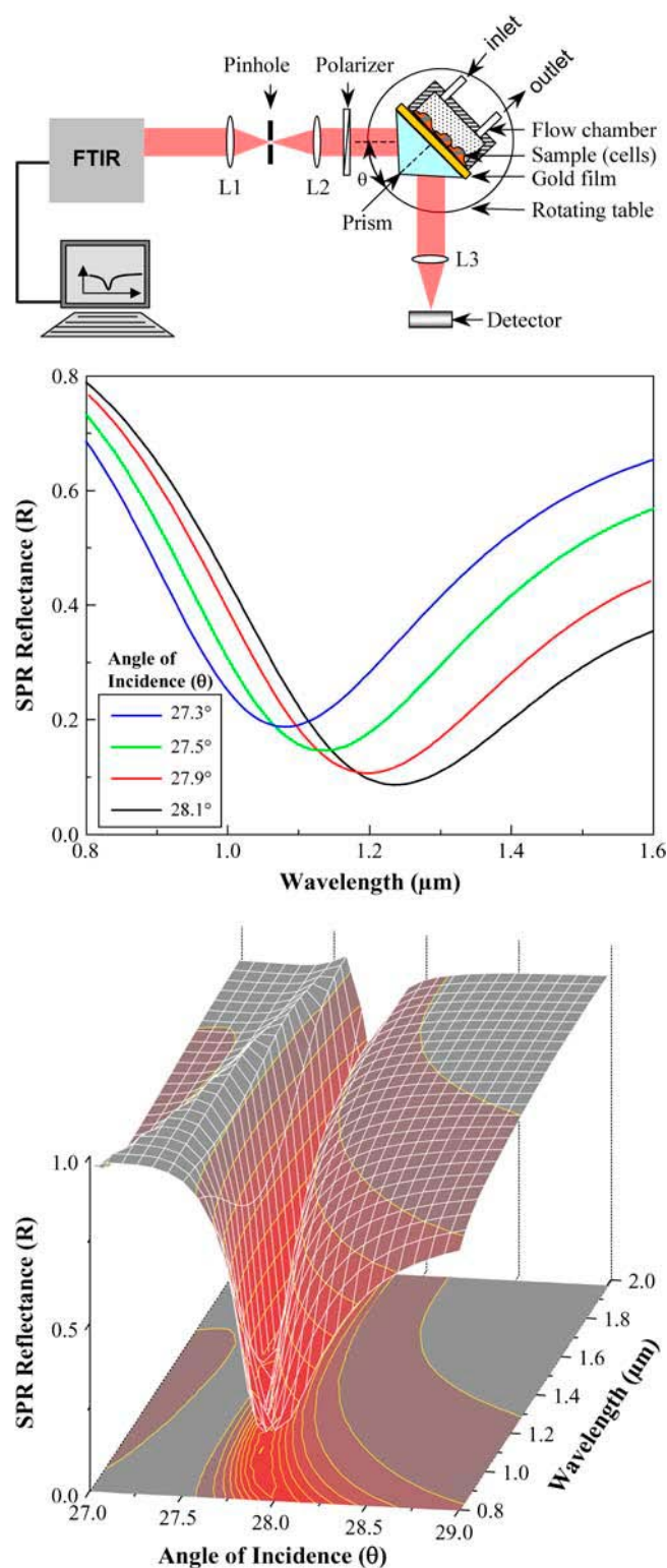
FIGURE 1 FTIR-SPR experimental setup. ( Upper panel ) Living cells were cultured onto a thin metallic (gold) film that coated a glass prism. The sample was illuminated with a collimated polarized IR light beam emitted from the FTIR spectrometer. During the measurements, the cells were in continuous contact with growth medium that filled the flow chamber. ( Middle panel ) Representative curves of FTIR-SPR reflectivity versus wavelength for the Au/air interface and for several angles of incidence, \theta
