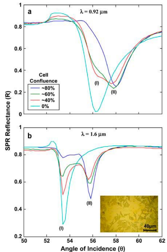
FIGURE 3 FTIR-SPR reflectance versus external angle from an Au-free or HeLa cell-occupied Au surface. Cells were cultured under conditions yielding \sim 80\% (blue), \sim 60\% (green), and \sim 40\% (red) cell occupancy of the gold-coated surface. Zero percent refers to an empty gold-coated prism subjected to cell growth medium (cyan). The degree of cell confluence was quantified with respect to the surface area occupied by the cells in a given microscopic field using images taken by phase contrast microscopy. A representative image of \sim 40\% cell coverage is shown in the inset of panel b . These data fully correlated with the degree of cell surface coverage estimated by FTIR-SPR scans (see text). FTIR-SPR measurements were performed at \lambda = 0.92 \mu\text{m} (panel a ) or 1.6 \mu\text{m} (panel b ). Two SPR minima denoted as (I) and (II) were seen only when the Au surface was partly occupied with cells. These minima were clearly resolved only at the higher wavelength (panel b ).
